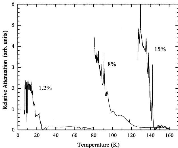
FIG. 4. Relative attenuation for three compositions of KTN.
